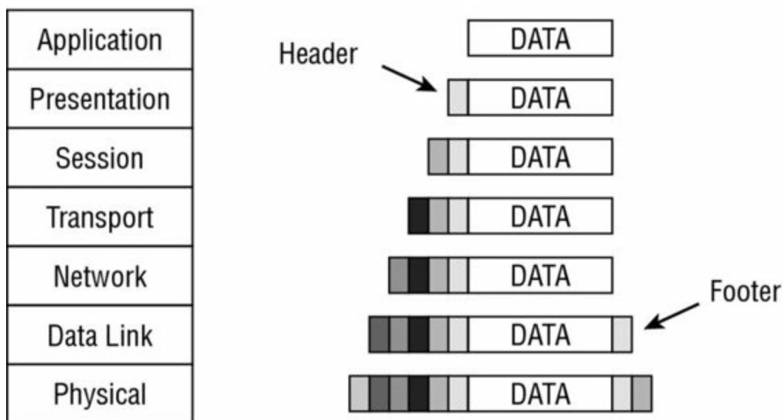
Figure 11.2 Representation of OSI model encapsulation
