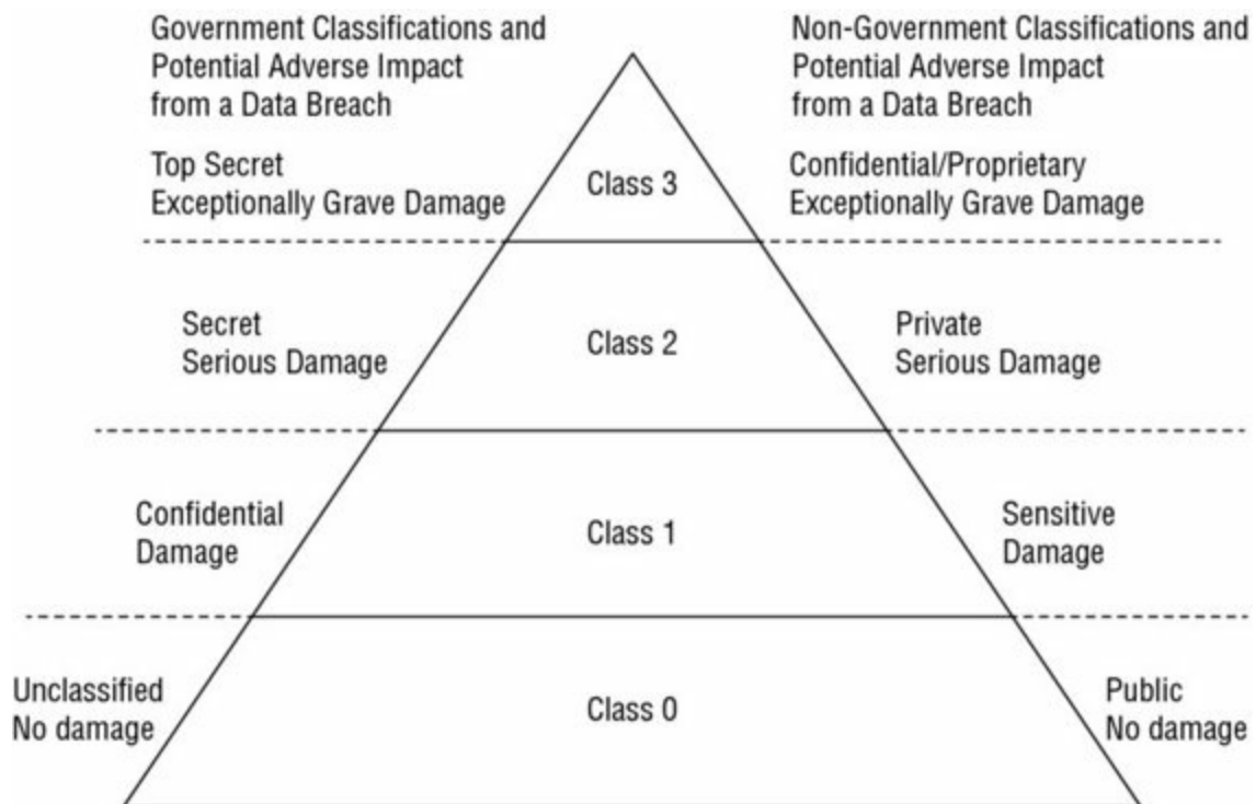
Figure 5.1 Data classifications
