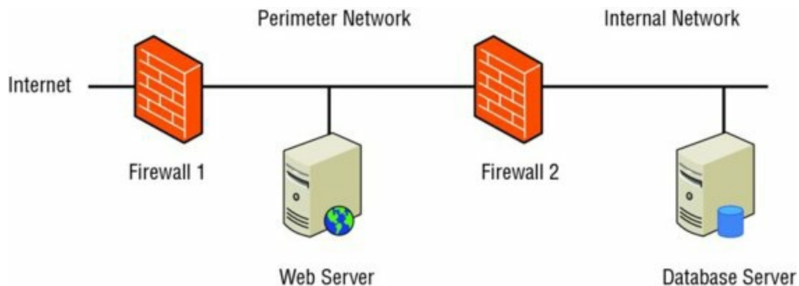
Figure 16.3 Web server and database server
