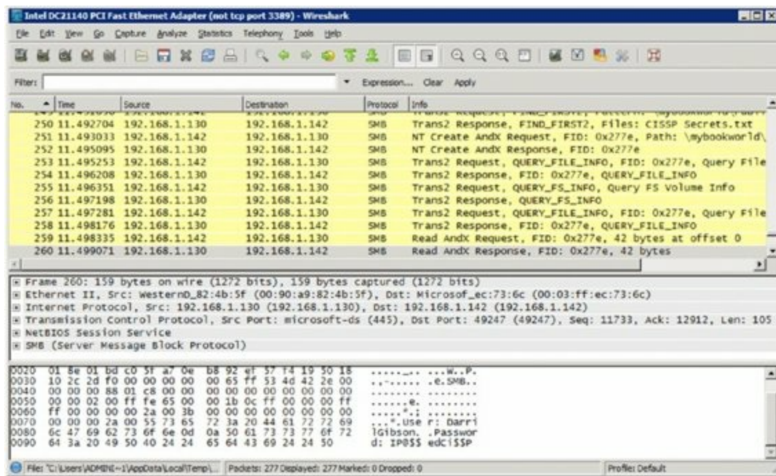
Figure 14.4 Wireshark capture
